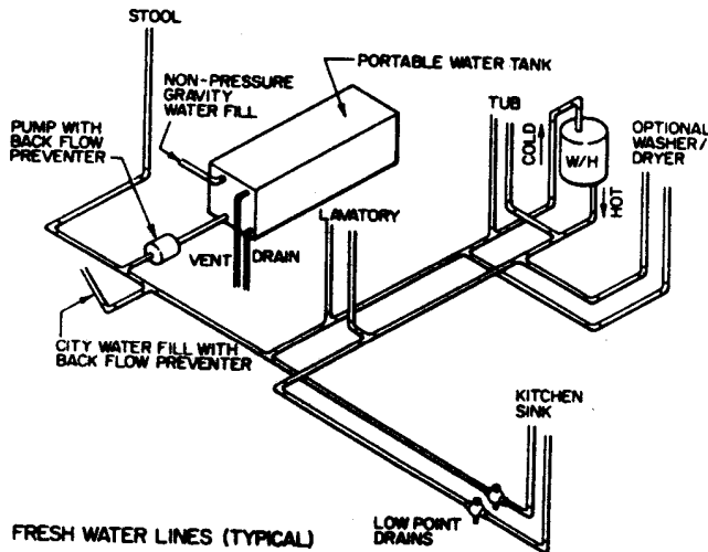
(FIG. 13) FRESH WATER LINES (TYPICAL)
