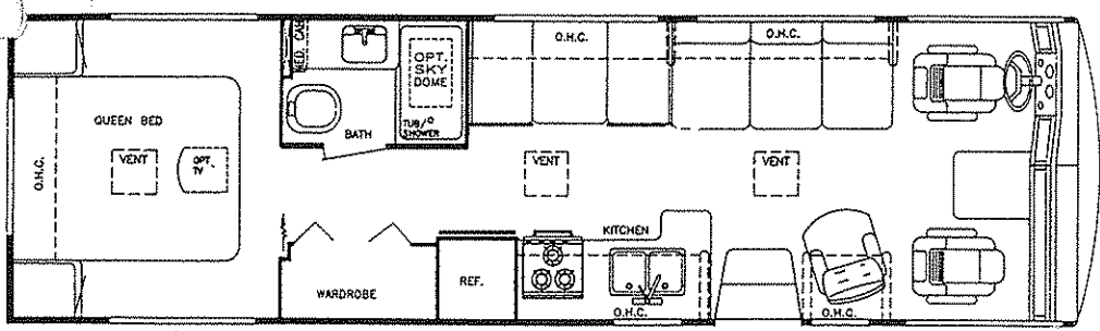
Model 8317 GAS
