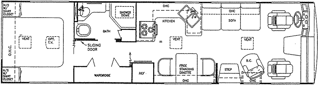
Model 8349 GAS
