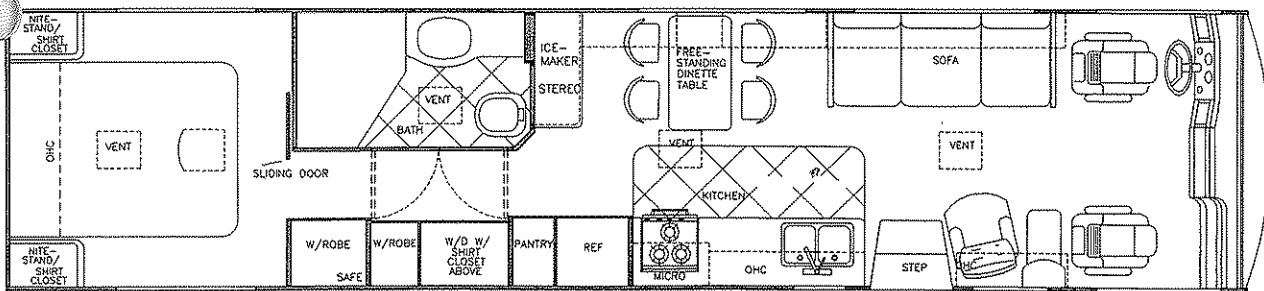
Model 8380 DIESEL
