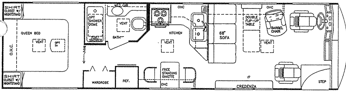
Model 8340 DIESEL
